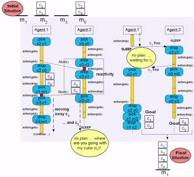
Fig. 5. Simulation trace example
