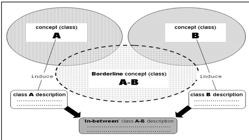
Fig. 1. The diagram presents an in-between or borderline concept, which lies between concepts A and B. The shaded area corresponds to the new concept description. SIR supports learning of the “in-between” concept description.
