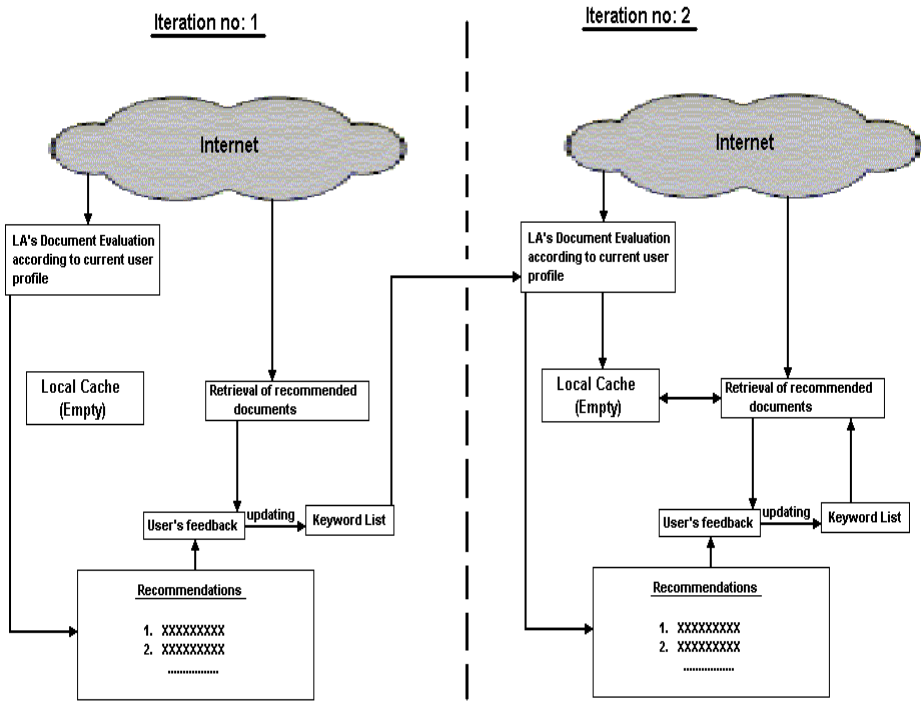
Fig. 4. Prefetching of the learning agent's recommendations. The procedure is repeated in the same way for more than two iterations
