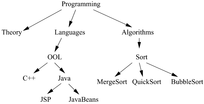
Fig. 1. A taxonomy
