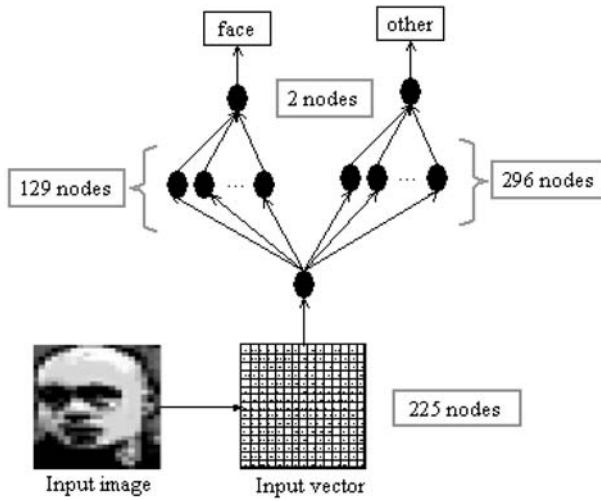
Fig. 6. PNN's architecture
