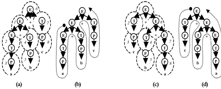
Fig. 1. (a) A tree constructed using Earley's parser for G CFG (b) Equivalent tree traversal for G CFG (c) A tree constructed using Earley's parser for G' CFG (d) Equivalent tree traversal for G' CFG.
