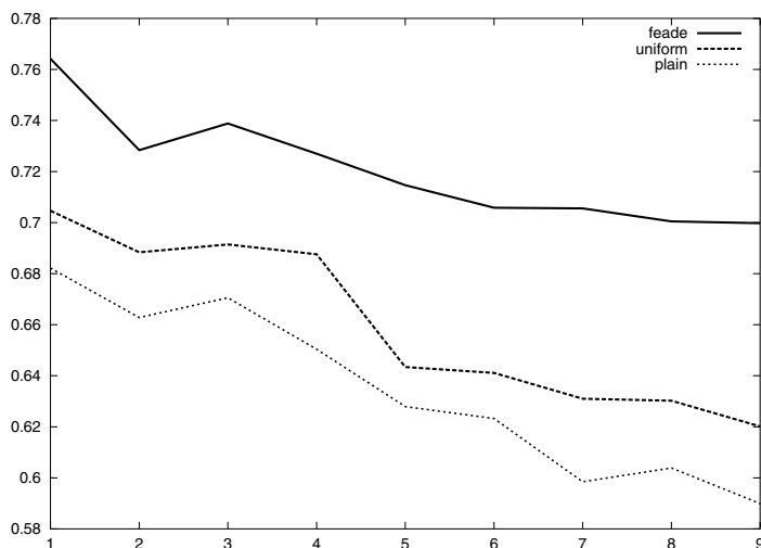
Fig. 2. Classification Accuracy of the K-NN algorithm for the “glass” dataset as a function of the number of nearest neighbors
