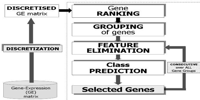
Fig. 2. The Gene-Selection process.
