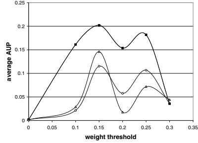
Fig. 3. Results for topics R10/R32(II)
