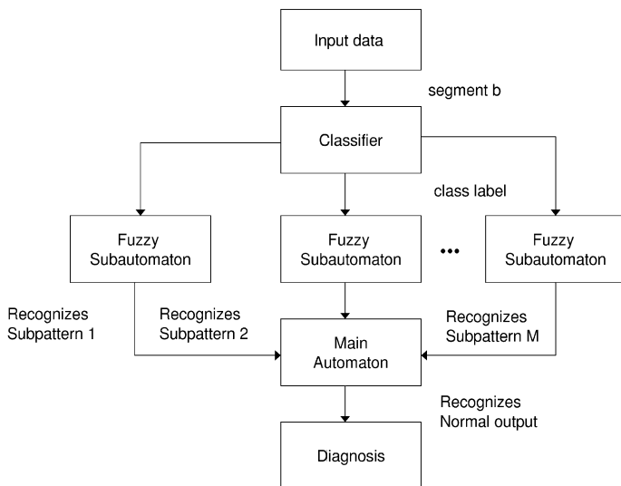
Fig. 2. System for automated fault diagnosis
