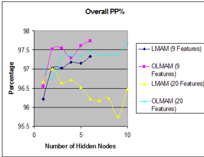
(c) PP% for LMAM and OLMAM with various number of features and hidden nodes.
