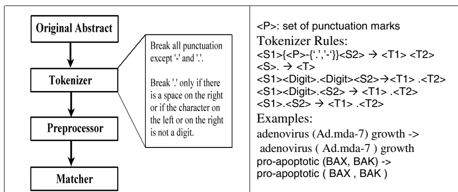
Fig. 1. Flowchart of the proposed molecular-biology names detector (left), the tokenization rules and two examples (right).
