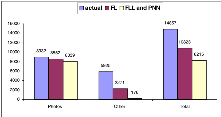
Fig. 7. Information Reduction/Loss
