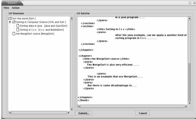
Fig. 3. Inferring annotation in XANNOT
